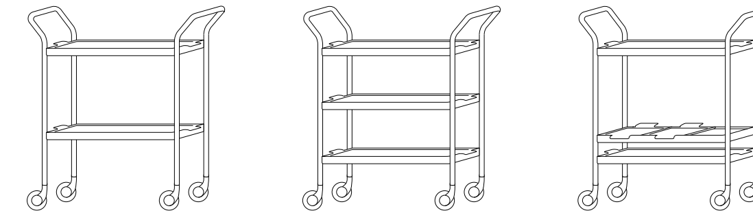
2519 Two Tier 535x355x650 mm (excl. handles) 3519 Three Tier 535x355x650 mm (excl. handles) C/3519 Drinks Trolley 535x355x650 mm (excl. handles)
